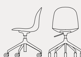
CB2175 61x57 H92(81) HS54(43) cm
